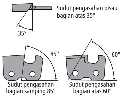
Gambar 6-15 Tipe semi pahat (semi-chisel)
