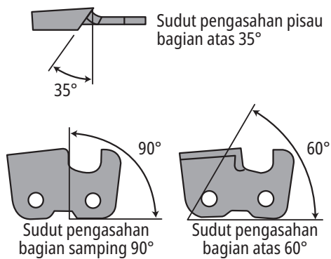
Gambar 6-13 Tipe chipper
