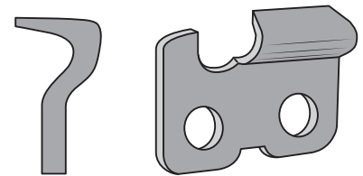
Gambar 6-8 Tipe semi pahat (semi-chisel)
