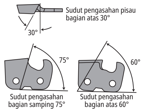
Gambar 6-14 Tipe pahat (chisel)
