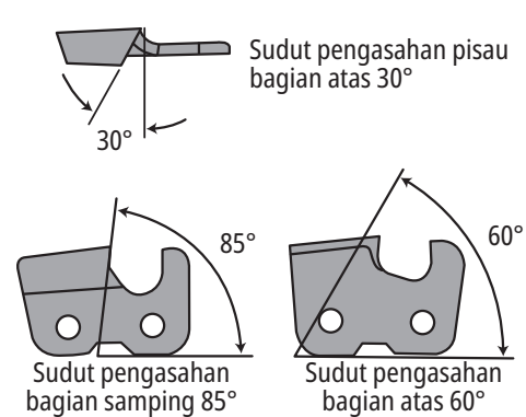
Gambar 6-16 Tipe micro-chisel
