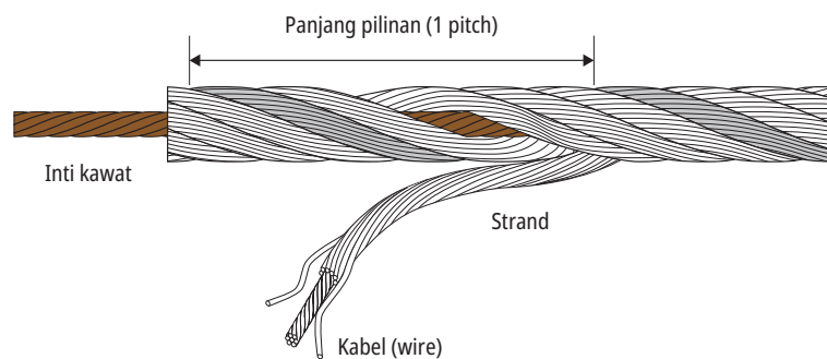
Gambar 7-11 Panjang pilinan tali kawat (1 pitch)
