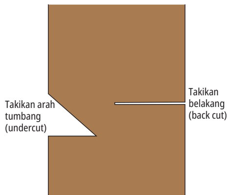
Gambar 10-15 Takikan arah tumbang (undercut), takikan belakang (back cut)
