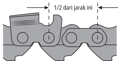
Gambar 6-10 Pitch
