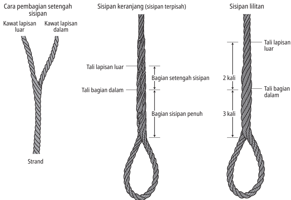
Gambar 7-12 Metode pengolahan eye splice – Sisipan keranjang (kagosashi), sisipan lilitan (makisashi)
