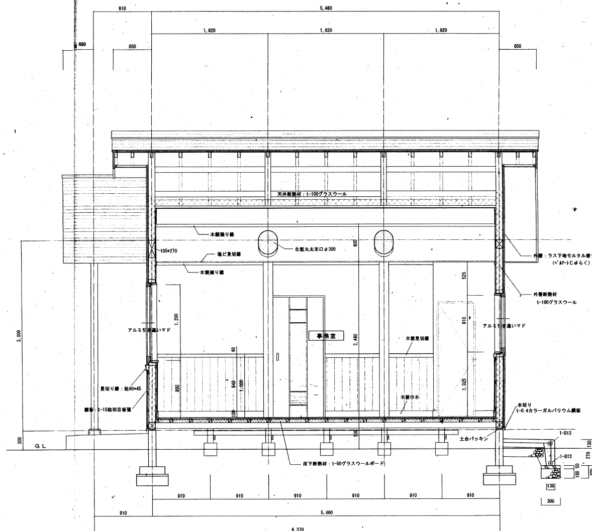
矩計図-2
