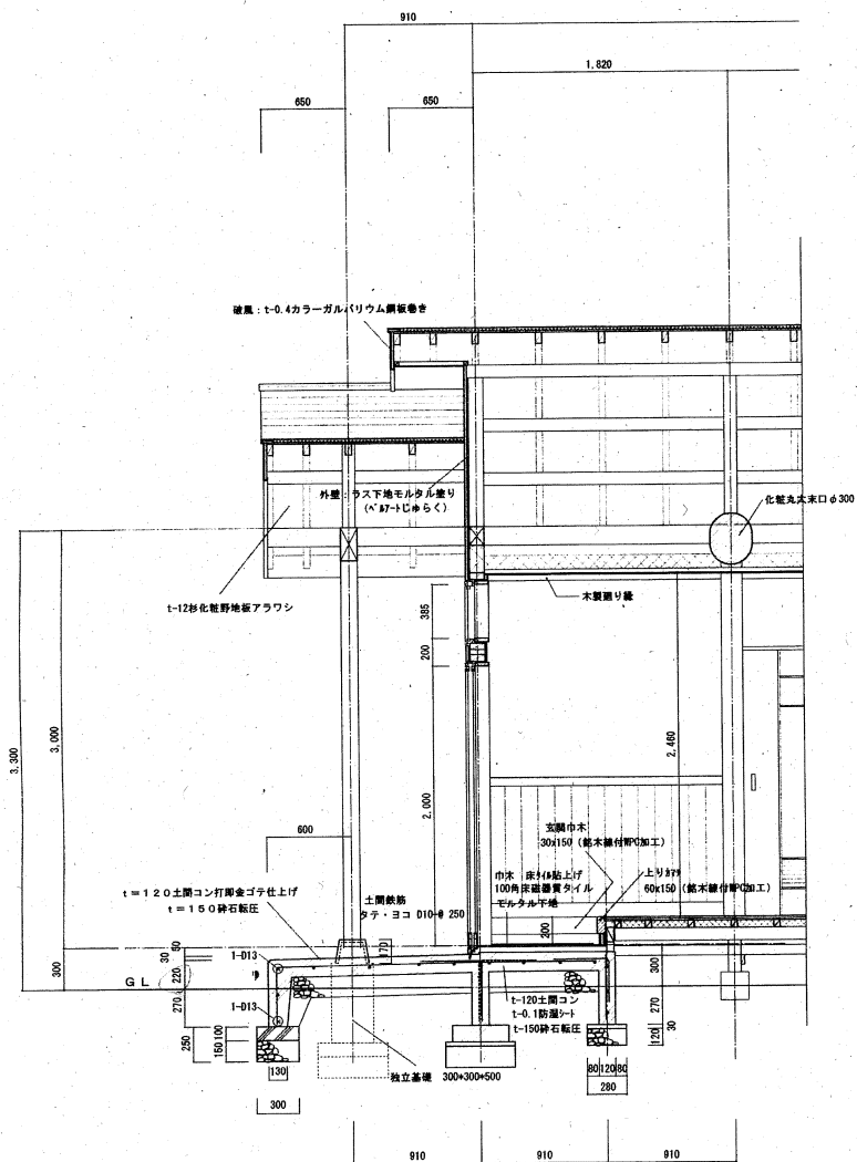
矩計図-3
